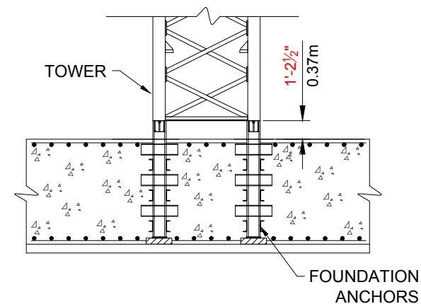
Elevation View of Anchors *Dimensions pertaining to 22.6 anchor
