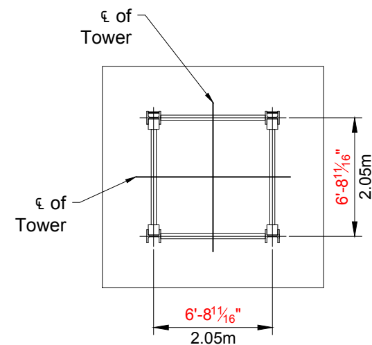
Plan View of Anchors
